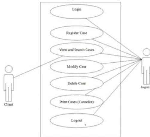
Fig 01: Use-case Diagram
